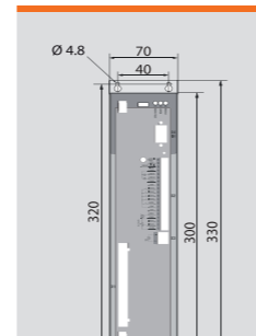
size 3 - Wall mounted
