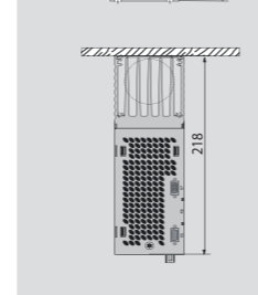
size 3 - Wall mounted
